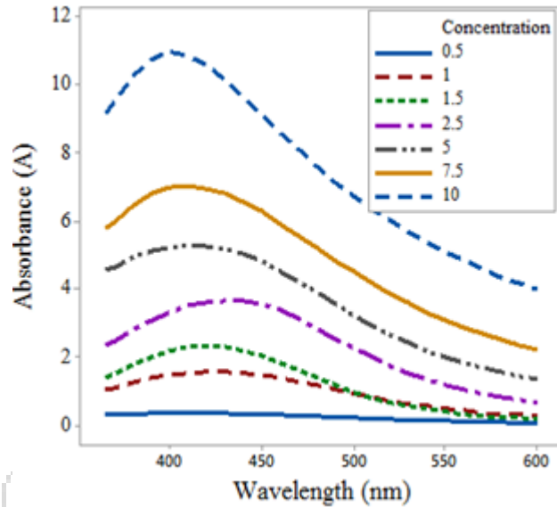
Fig.6 Effect of \text{AgNO}_3 Concentration (mM)
