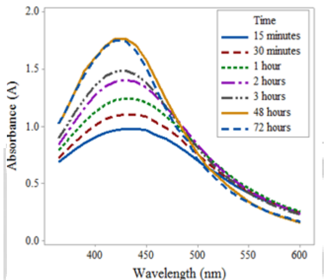
Fig.5 Increasing absorbance of SPR peak as the time increased.
