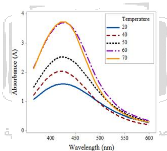
Fig.7 Increasing absorbance of SPR peak as temperature (°C) increased.
