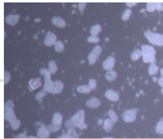
Fig. 7 Microscopic View and Comparative Particle Size Distribution (PSD) of New PA12 Powder.
